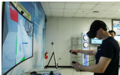
Virtual Reality
