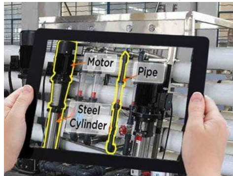
Augmented Reality
